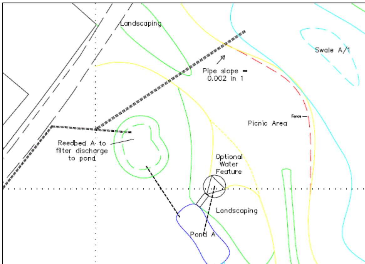
Fig 3. Detail from plan, showing reedbed for treatment of influent regular rainfall from drain that conveys hard surface run-off, prior to discharge into pond – a bypass diverts major rainfall to swale.
