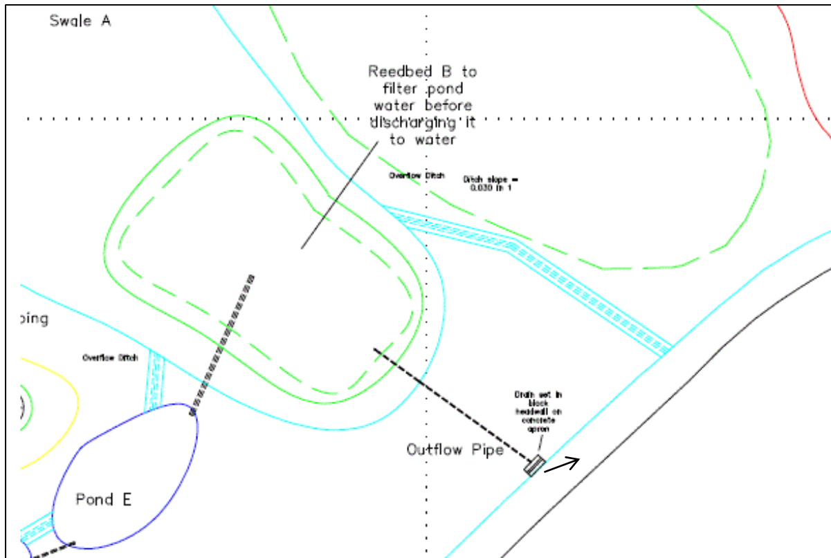
Fig 4. Detail from plan, showing reedbed for treatment of all outflows from swale, prior to discharge into ditch (and then into Normans Brook).
